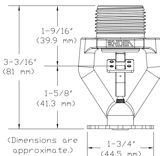
Figure 2: Pendent Sprinkler VK592 Dimensions
