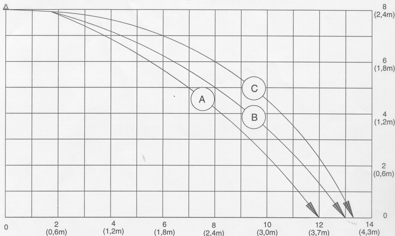
Typical front view of one half of the spray pattern produced by a Model B-2 Horizon Mirage Sprinkler
