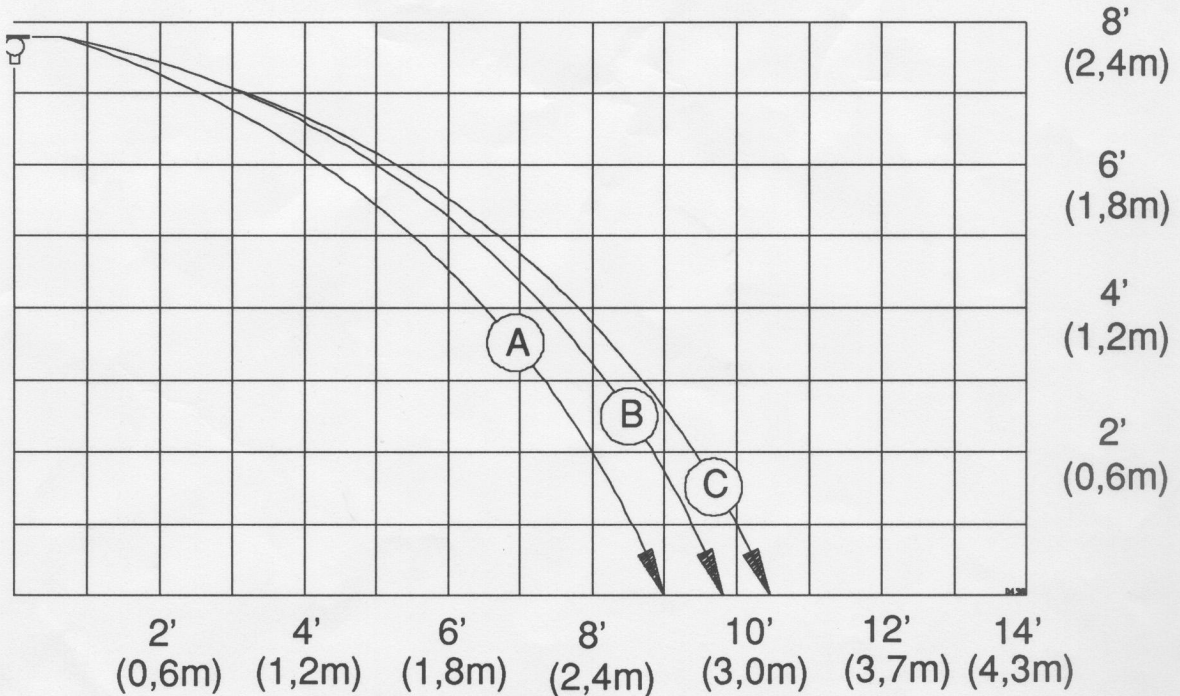
Typical profile of one half of the spray pattern produced by a Viking Micromatic Model M 1/2" European Upright Sprinkler.
