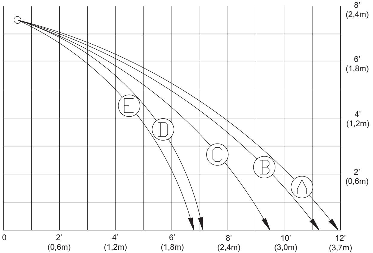
Typical profile of one half of the spray pattern produced by a Viking ESFR Pendent SIN VK503 Sprinkler (K=16.8)
